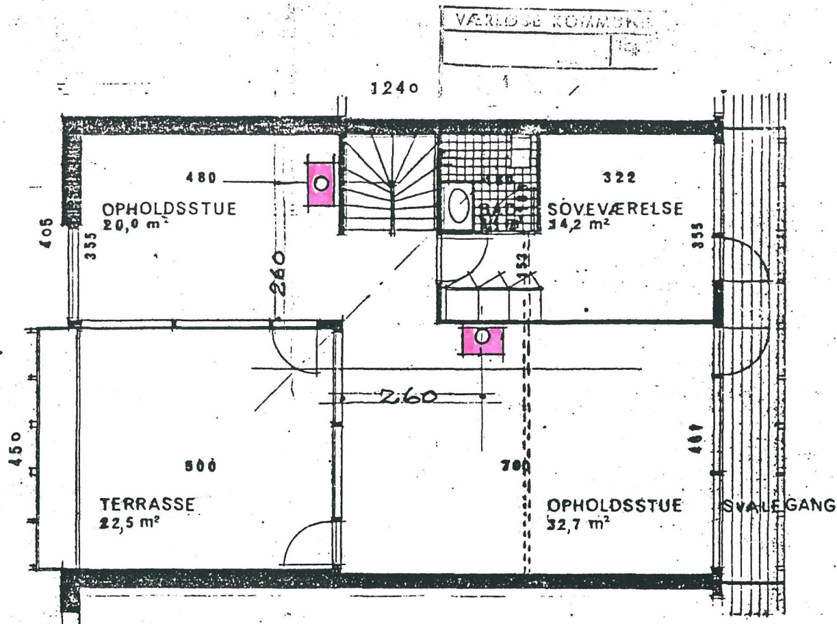
1. SAL' PLAN
