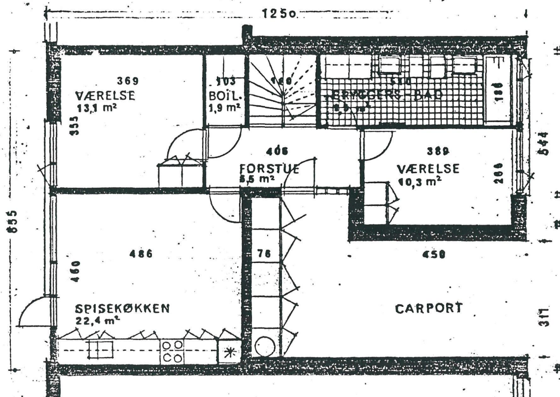
1. SAL' PLAN
